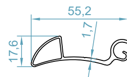
تیغه ابتدایی Primary Shutter code: 9103
