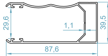
ريل كستل Castle Rail Profile code: 9151
