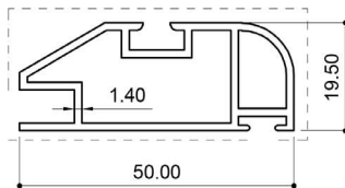
21244 (0.632 Kg/m)
