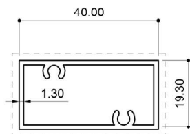
20101 (0.470 Kg/m)
