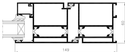
door profile MB-60
