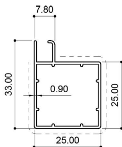
21515 (0.291Kg/m)
