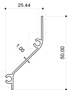
12624* (0.221 Kg/m)
