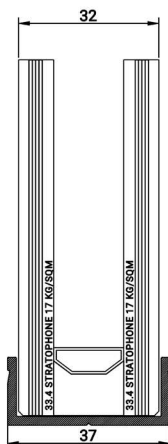
FS 3254 SINGLE GLASS ADAPTOR WEIGHT 0.526 KG/M
