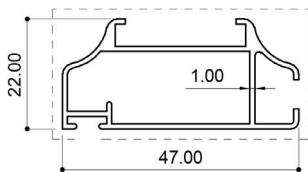
22396 (0.428 Kg/m)
