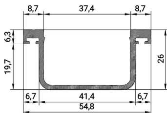
FS 3225 SINGLE RAIL INTERLOCK WEIGHT 0.631 KG/M
