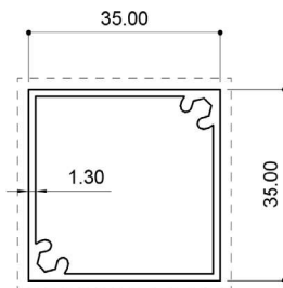
20622 (0.554 Kg/m)
