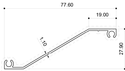
14590 (0.330 Kg/m)
