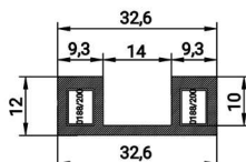
FS 3248 SINGLE GLASS ADAPTOR WEIGHT 0.450 KG/M
