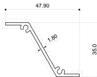
10248 (0.397 Kg/m)
