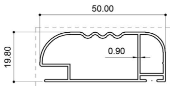
26028 (0.397 Kg/m)
