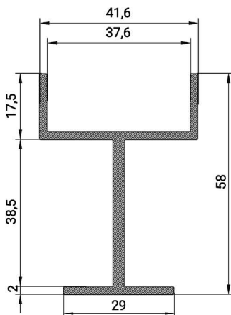
FS 3273 STONE SILL PROFILE WEIGHT 0.860 KG/M
