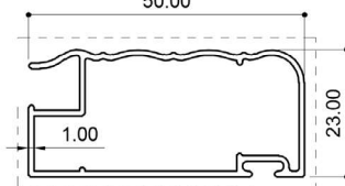
22117 (0.439 Kg/m)
