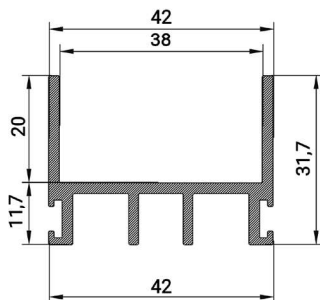
FS 3274 STONE SILL PROFILE WEIGHT 0.688 KG/M
