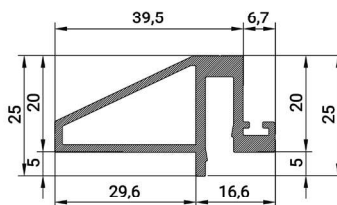
FS 3229 SINGLE RAIL WALL COVER WEIGHT 0.682 KG/M
