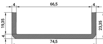
FS 3226 SINGLE RAIL INSTALLATION PROFILE WEIGHT 1.196 KG/M
