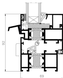
window profile MB-60HI
