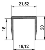
BP 002 BALAUSTRADE TOP PROFILE WEIGHT 0.253 KG/M
