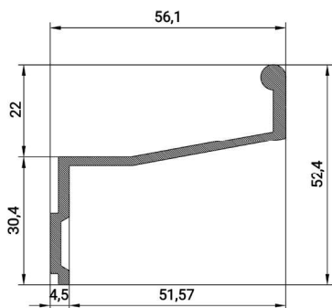
FS 3266 HANDLE FOR CLOSING INVERSION WEIGHT 0.668 KG/M
