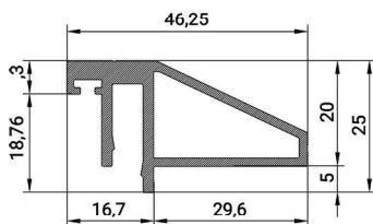
FS 3230 SINGLE RAIL WALL COVER WEIGHT 0.682 KG/M
