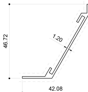
11436 (0.294 Kg/m)
