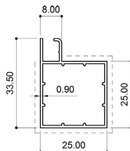
24813 (0.296 Kg/m)
