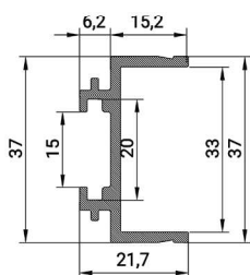
FS 3210 LATCHING HANDLE PROFILE POLYCARBONATE
