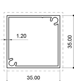
26022 (0.481 Kg/m)
