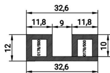
FS 3254 SINGLE GLASS ADAPTOR WEIGHT 0.526 KG/M
