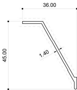
10102 (0.253 Kg/m)
