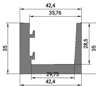
BP 002.1 BALAUSTRADE SILL PROFILE WEIGHT 0.634 KG/M
