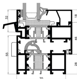
window profile MB-70 HI
