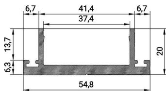
FS 3227 SINGLE RAIL INTERLOCK WEIGHT 0.818 KG/M
