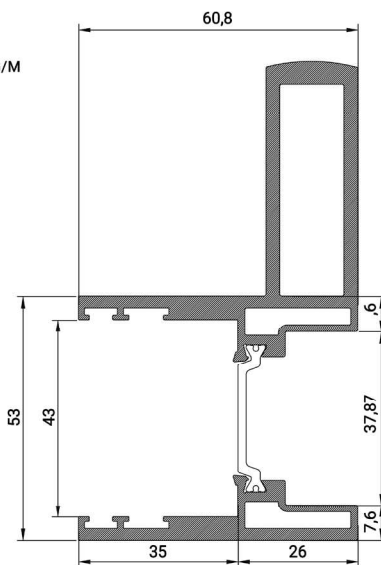
FS 3239401 4TH PANELS HANDLE PROFILE WEIGHT 2.614 KG/M
