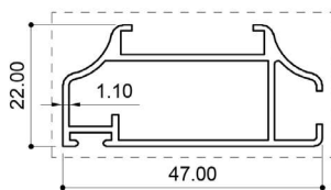
21077 (0.466 Kg/m)
