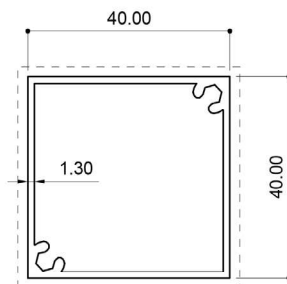
20621 (0.624 Kg/m)
