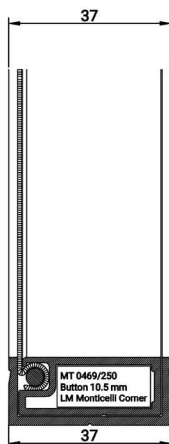
FS 3255 FLY SCREEN ADAPTOR WEIGHT 0.381 KG/M
