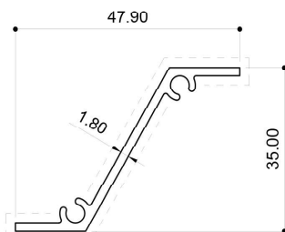
11692 (0.379 Kg/m)
