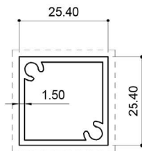
20104 (0.447 Kg/m)
