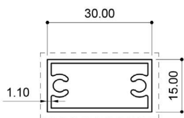
21161* (0.342 Kg/m)
