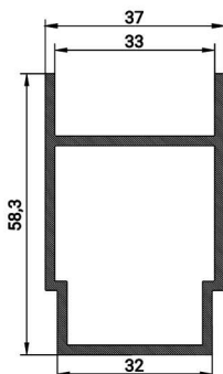
FS 3253 KEY LOCKS PROFILE WEIGHT 0.986 KG/M
