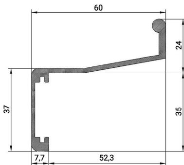
FS 3246 HANDLE FOR MULTIPOINT CLOSING WEIGHT 0.767 KG/M
