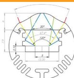
Alu-Round profile with 30° lens LEDs type 5060
