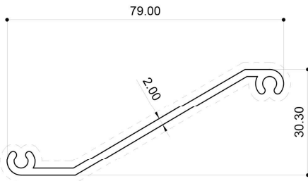
11417 (0.562 Kg/m)
