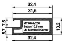
FS 3255 FLY SCREEN ADAPTOR WEIGHT 0.381 KG/M
