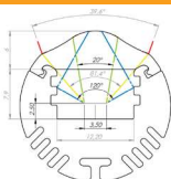
Alu-Round profile with 30° lens LEDs type 3528
