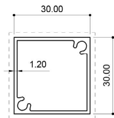
22634 (0.425 Kg/m)
