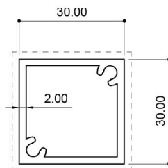
20014 (0.664 Kg/m)
