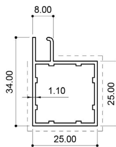
23700 (0.371 Kg/m)
