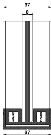
FS 3248 SINGLE GLASS ADAPTOR WEIGHT 0.450 KG/M
